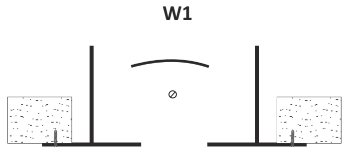
Visible assembly using screws and the mounting holes in the diffuser frame.
